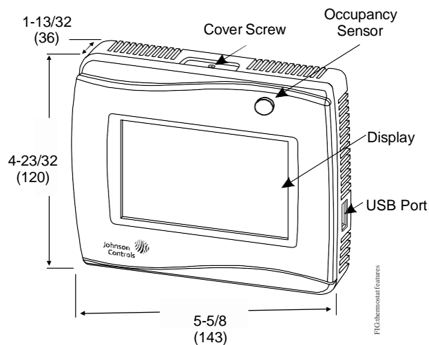
TEC3000 Series Thermostat Controller Shown with Occupancy Sensor, Dimensions, in. (mm)
