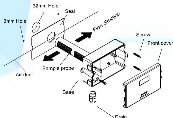
Duct mount installation
